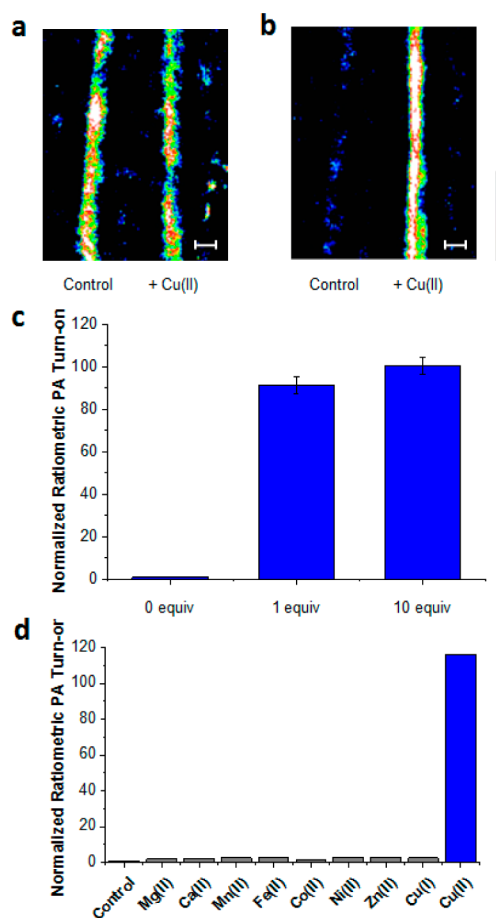
Figure 4. Photoacoustic imaging of APC-2 treated with Cu(II). Photoacoustic images of 10 \mu\text{M} APC-2 (PBS + 0.1% CrEL, pH 7.4) in FEP tubing overlaid with a 1 cm thick phantom treated with 0 and 10 equiv of Cu(II), with excitation at (a) 697 and (b) 767 nm. Pseudocoloring represents intensity distribution from highest intensity, indicated by white, to the lowest intensity, designated by black. Scale bar represents 2 mm. (c) Quantification of APC-2 treated with 0, 1, and 10 equiv of Cu(II) for 90 min. Blue bars represent normalized ratiometric turn-on responses calculated from the PA ratios (PA 767 /PA 697 ) for control and Cu(II)-treated conditions. n = 2 . (d) PA responses of APC-2 to various metal ions (2 mM for Ca(II) and Mg(II), 50 \mu\text{M} for all other cations).
